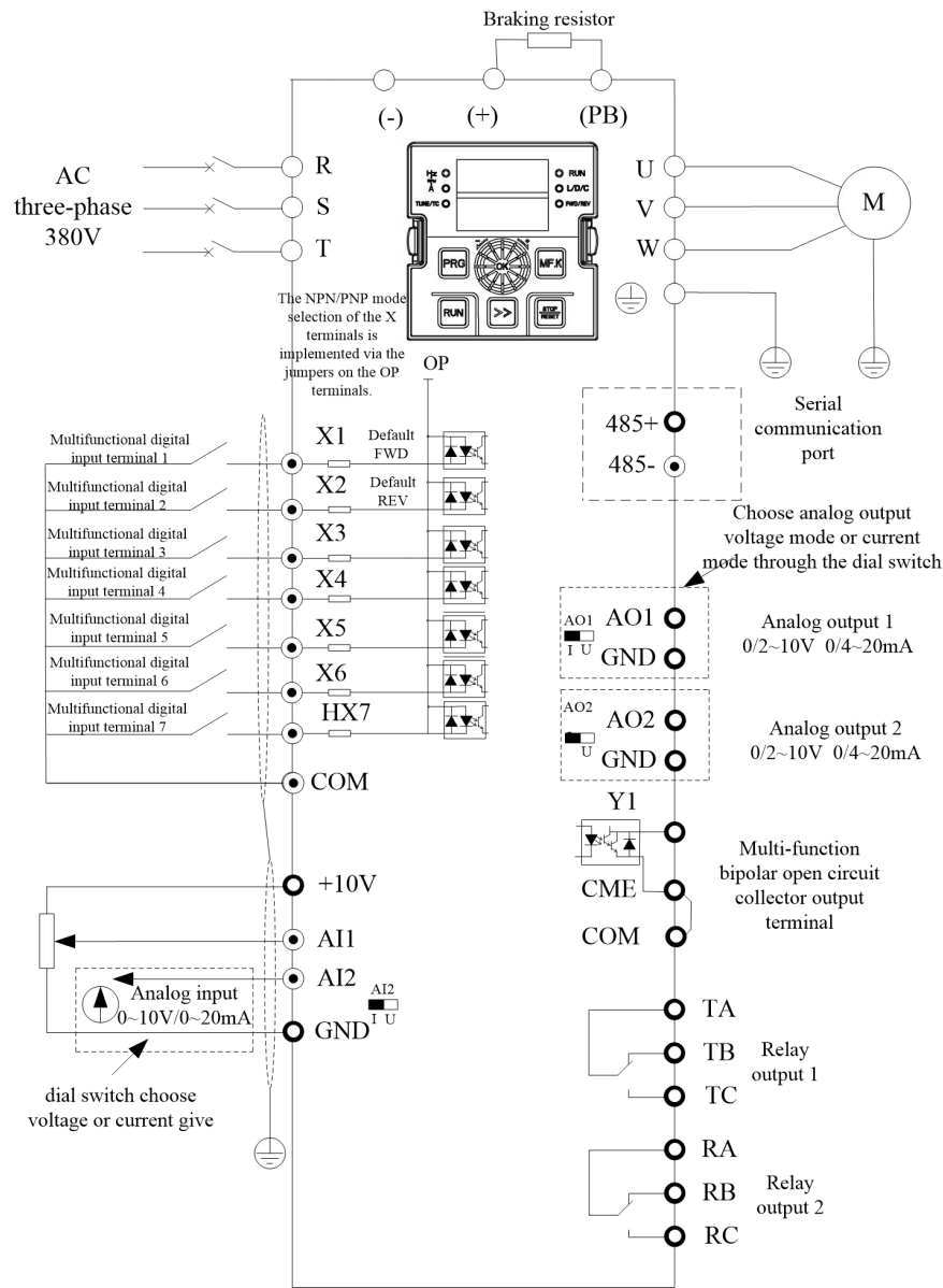
Figure 3-2. Three-phase 380V 4.0 to 30kW (4T:380V) and single-phase 220V (3S) 5.5kW or less (input connected to R T) Inverter Wiring Diagrams Note: The dip switch for the digital input terminal X is factory-set to NPN mode (with the OP terminal connected to the 24V terminal by default), meaning the connection between terminal X and COM is active when short-circuited. The dip switches for AI2, AO1 and AO2 are factory-set to voltage mode by default.
