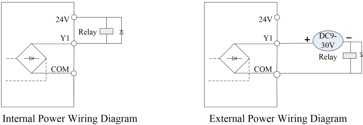
Figure 3-12. Digital Output Terminal Y1 Wiring Diagram
