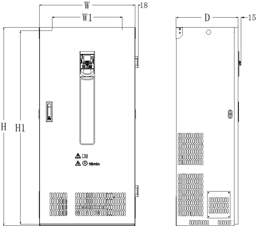
Figure 2-6. External/Mounting dimensions of inverter for 380V 220kW or more
